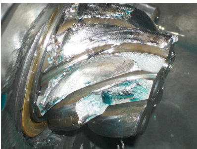
Missing teeth on the 911 pinion gear.
